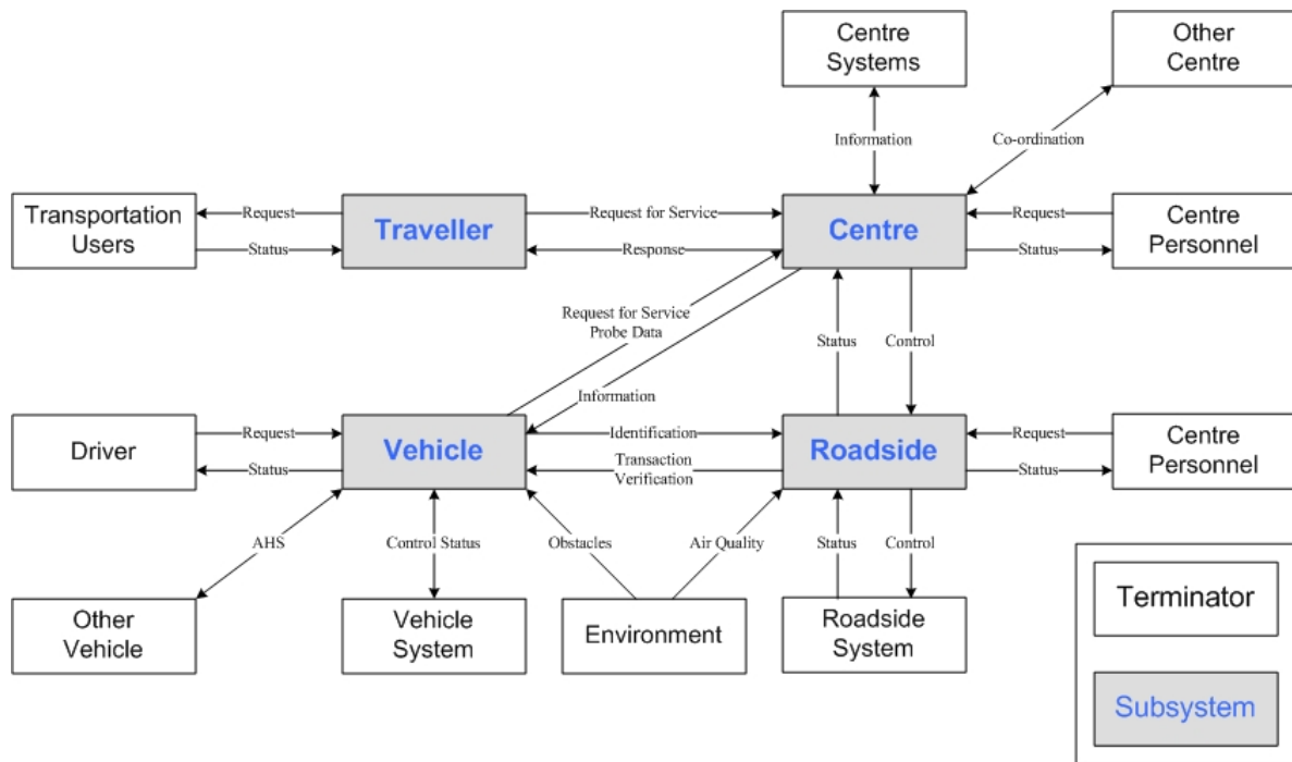
Figure 2 – Top Level Architecture Flow Diagram
